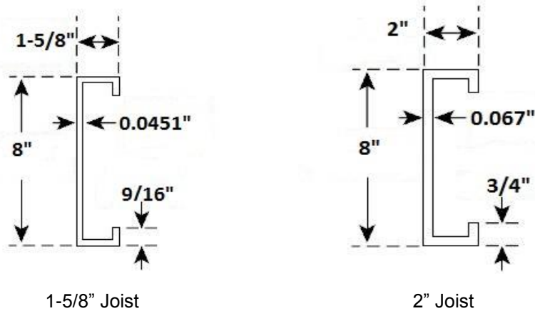
Figure 3 – Steel Joists
