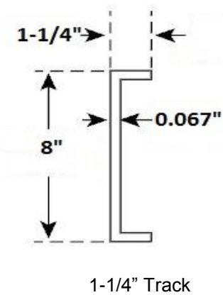
Figure 4 – Track/Ledger
