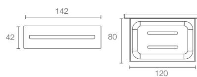
COMPLEMENTARY™ K-25068IN-CP
