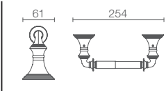
DEVONSHIRE® | K-10554-CP
