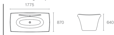
ESCALE™ | K-11344T-0
