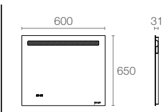
FOREFRONT™ | K-23265IN-NA
