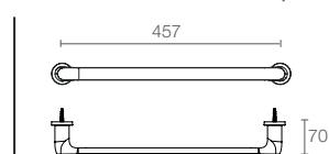
AVID™ | K-97494T-CP
