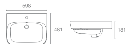
MODERNLIFE™ | K-77775T-1-0
