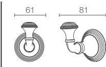
DEVONSHIRE® | K-10555-CP
