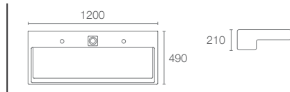
TERRACE™ | K-XB112K-00 *
