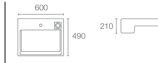
TERRACE™ | K-XE112K-00
