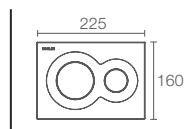
LYNK™ | K-75890IN-M-CP
