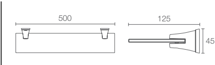
COMPLEMENTARY™ | K-5636IN-CP
