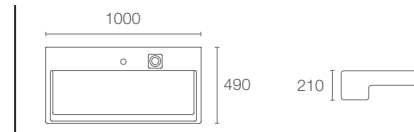
TERRACE™ | K-XC112K-00
