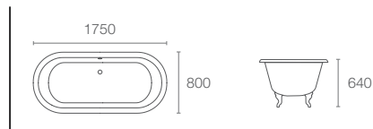
CLEO™ | K-11195T-0
