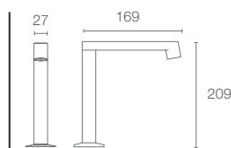
COMPONENTS™ | K-77969T-CP
