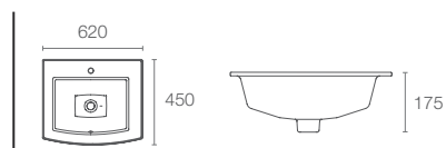
FOREFRONT™ | K-2949T-0
