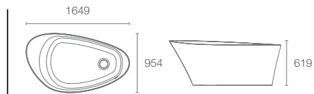
VEIL® | K-8331T-0
