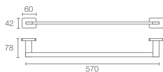
COMPLEMENTARY™ K-25065IN-CP
