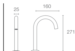
COMPONENTS™ | K-77967T-CP
