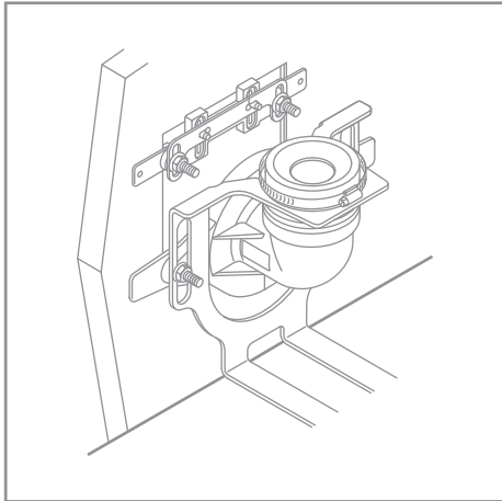
STEP 2 Install bracket and connector system to existing carrier in wall.
