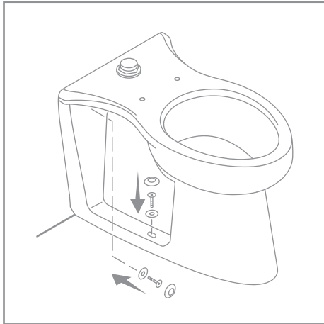
STEP 3 Place bowl onto connector system and secure in place.
