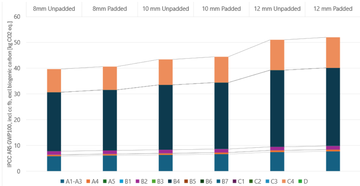
Figure 2: Contribution analysis for 8mm, 10mm, and 12mm Padded and Unpadded Laminate Flooring – TRACI 2.1
