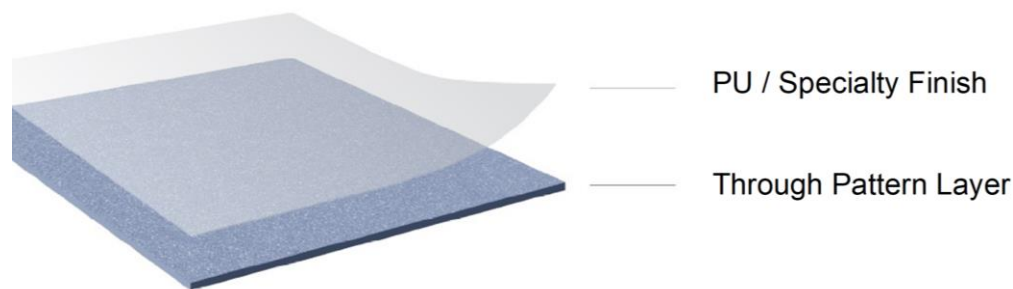
Figure 1. Cross-Section Diagram of Homogeneous Sheet Vinyl Flooring
