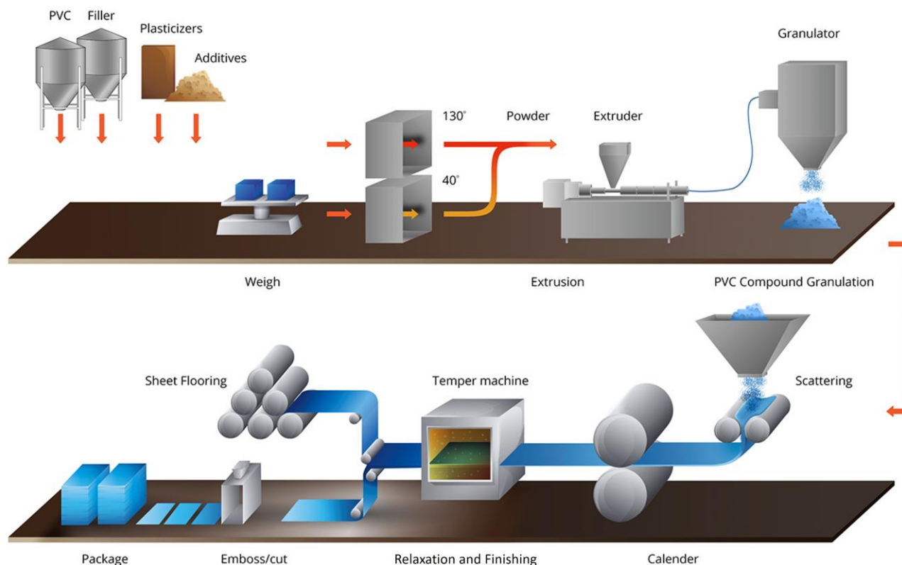
Example of Production Line for Homogeneous Sheet Vinyl Flooring
