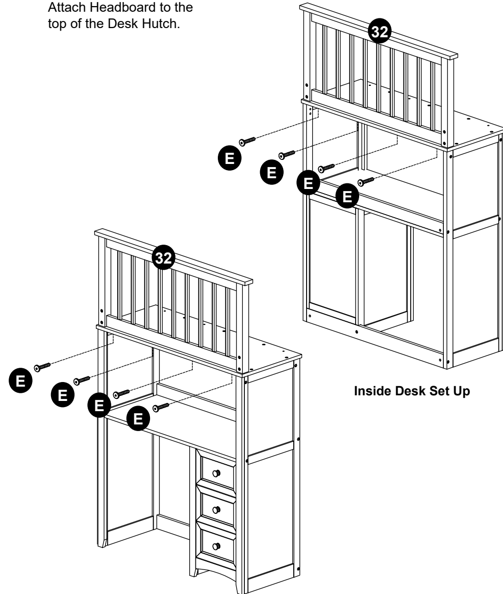
Outside Desk Set Up
